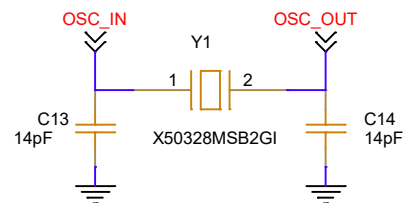
HIGH SPEED EXTERNAL CRYSTALL
